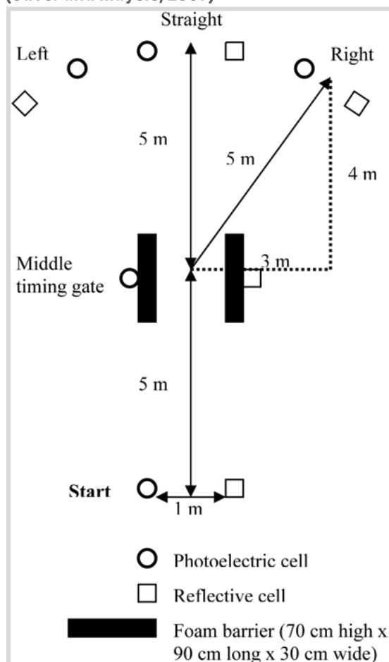
Figure 6: Planned or Reactive Agility Test Execution with Luminous Visual Stimuli (Oliver and Mayers, 2009)
